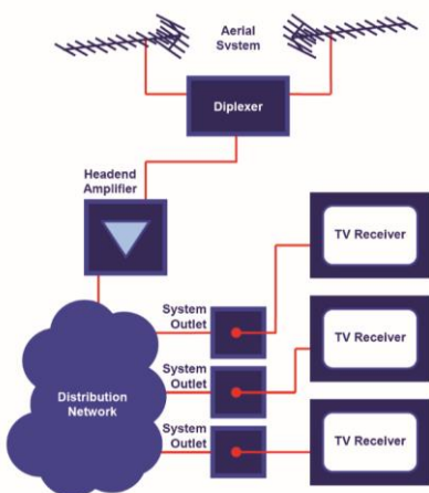
Figure 1: Block diagram of an MATV system
