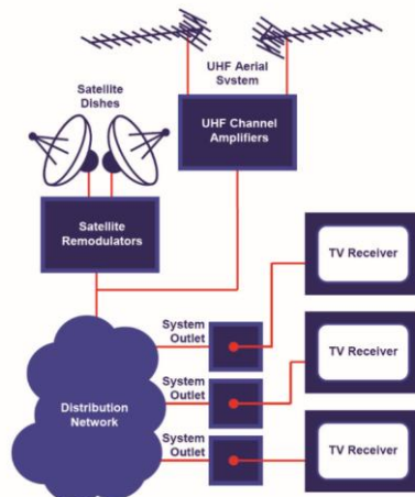
Figure 2: Block diagram of a SMATV system
