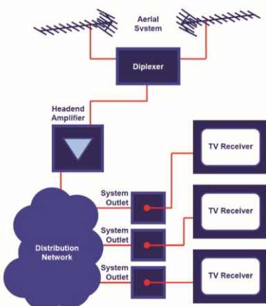
Figure 1: Block diagram of an MATV system
